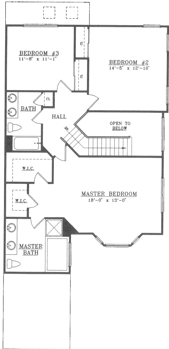
SECOND FLOOR
