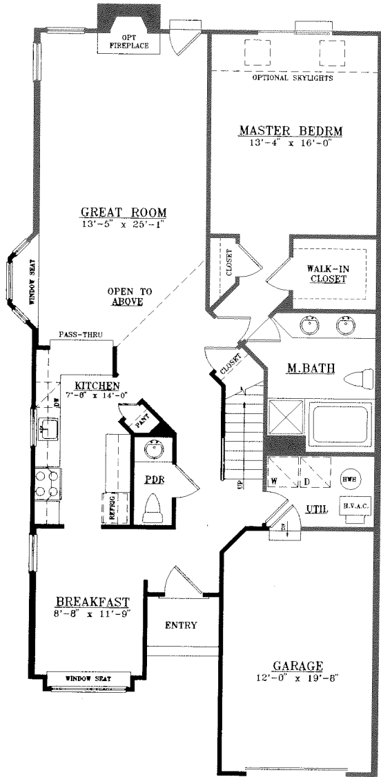
FIRST FLOOR
